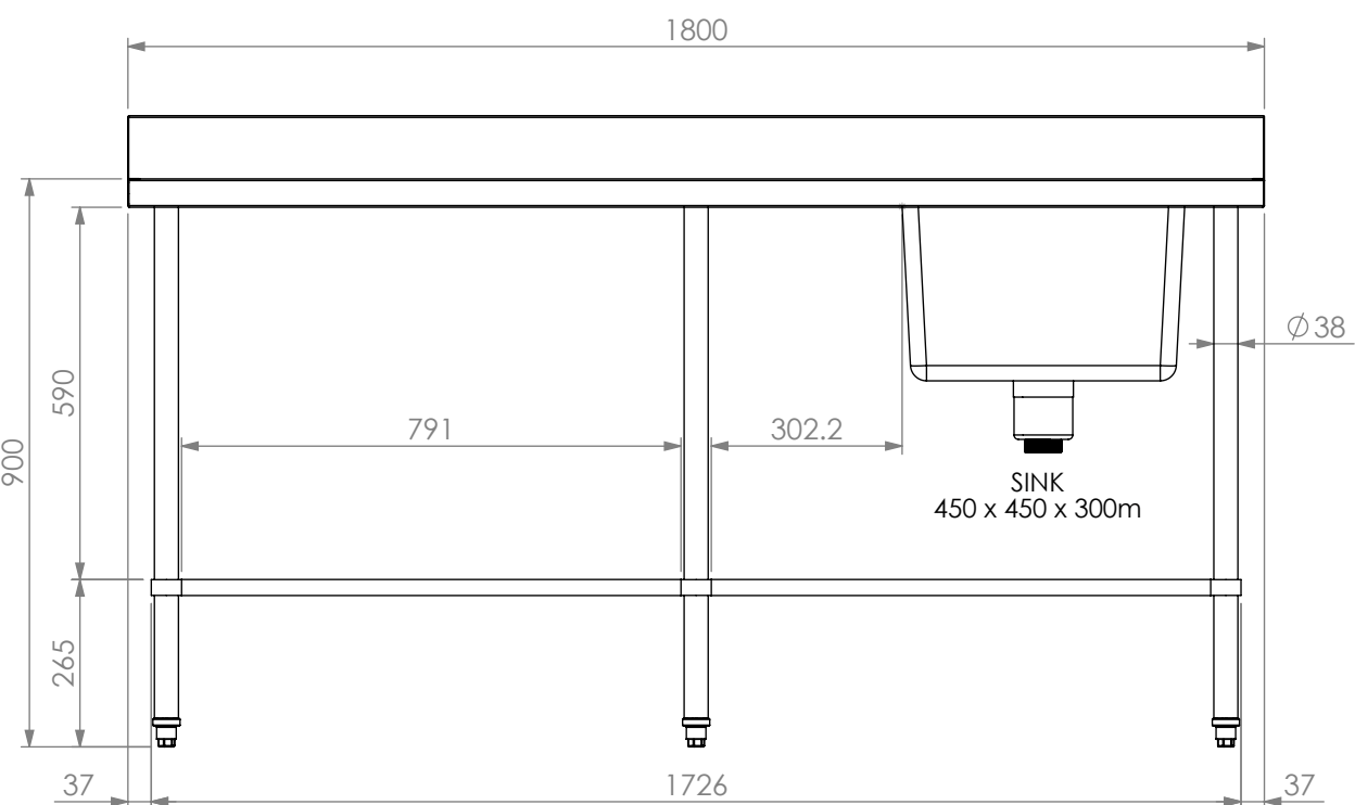
FRONT ELEVATION
