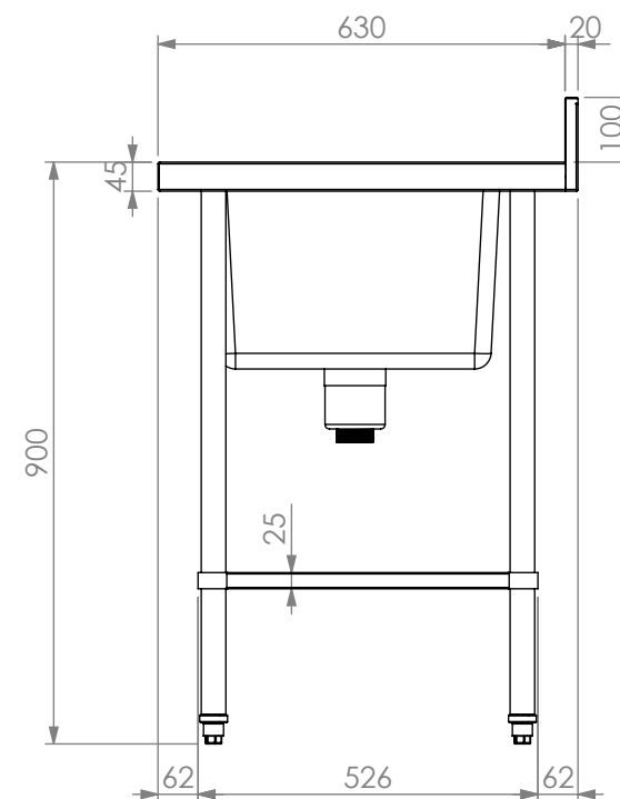
SIDE ELEVATION
